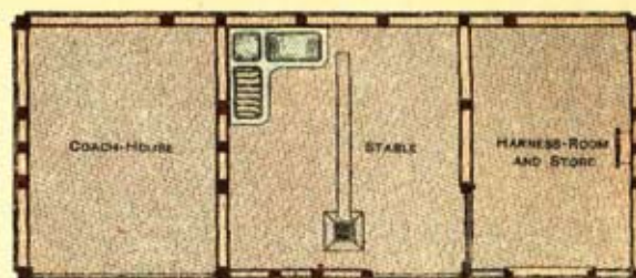
SECTIONAL PLAN
