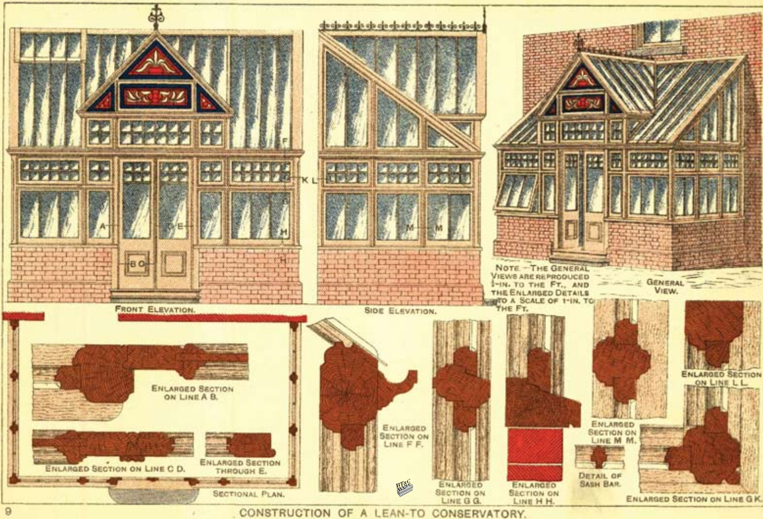
CONSTRUCTION OF A LEAN-TO CONSERVATORY.
