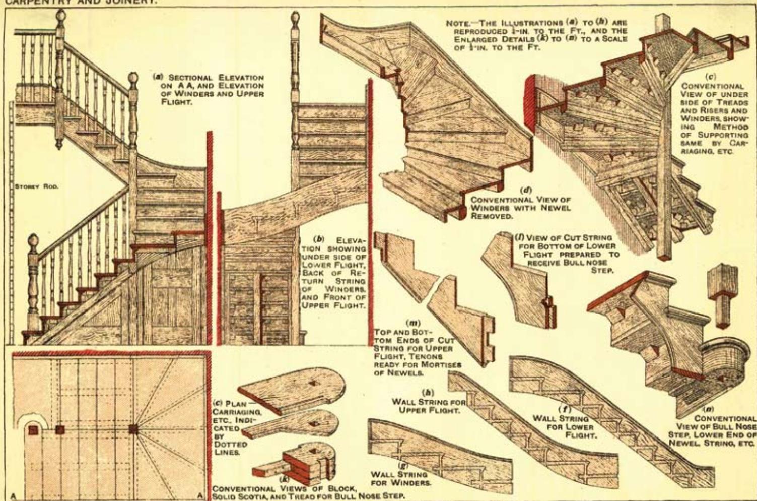
NEWEL STAIRCASE WITH WINDERS IN HALF SPACE.
