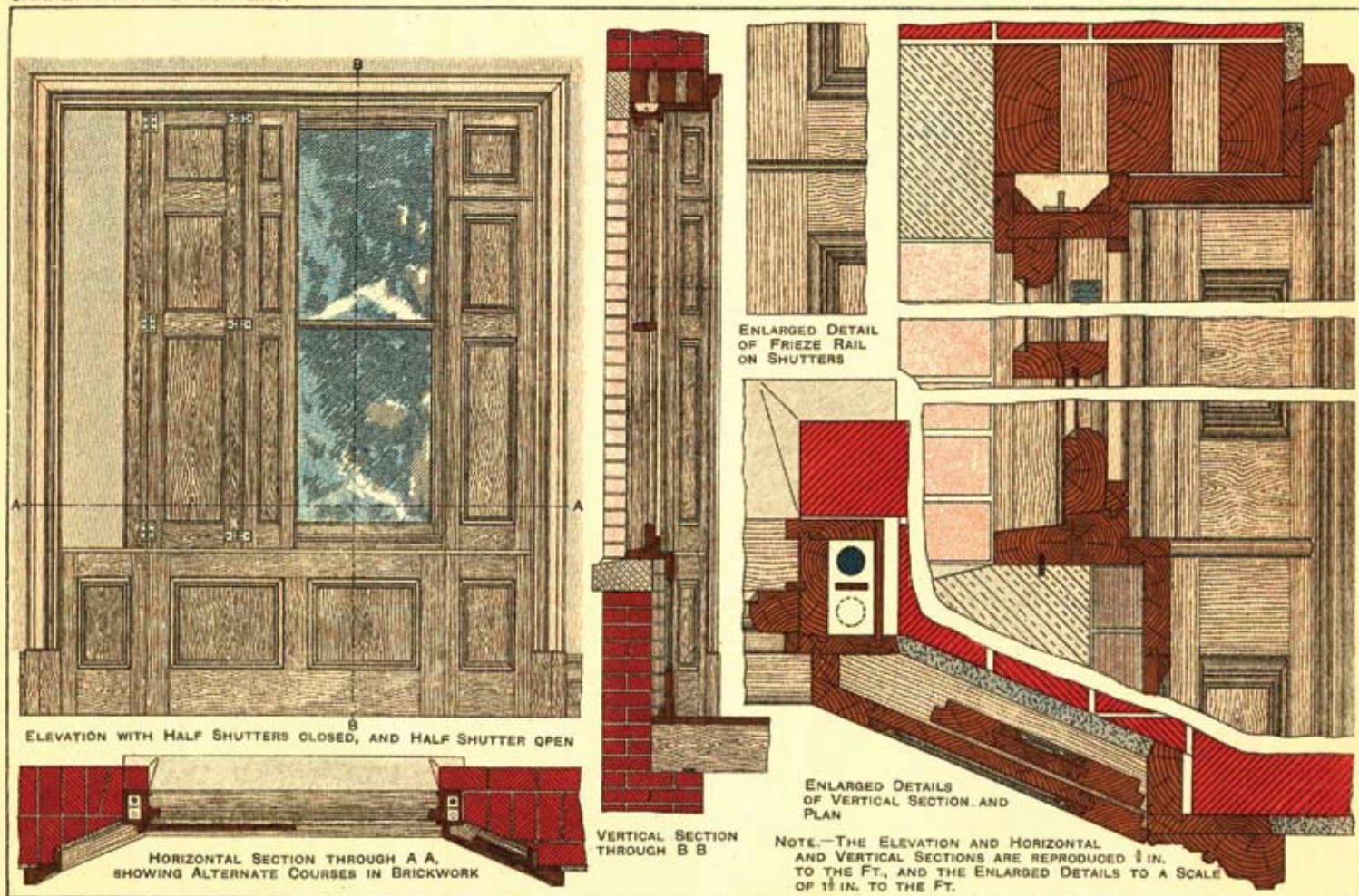
BOXING SHUTTERS TO SASH WINDOW
