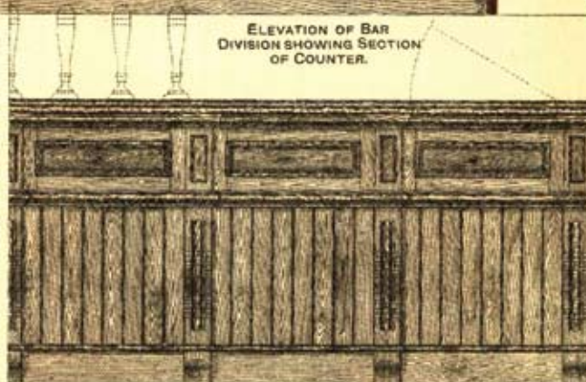
HALF ELEVATION OF BAR COUNTER.
